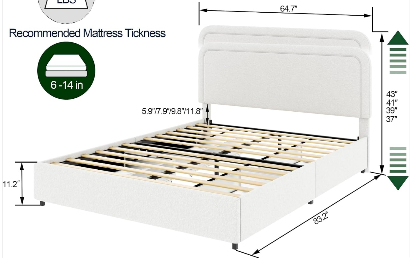
Image 8.1: Key dimensions and specifications of the Brabrety Queen Size Platform Bed.
