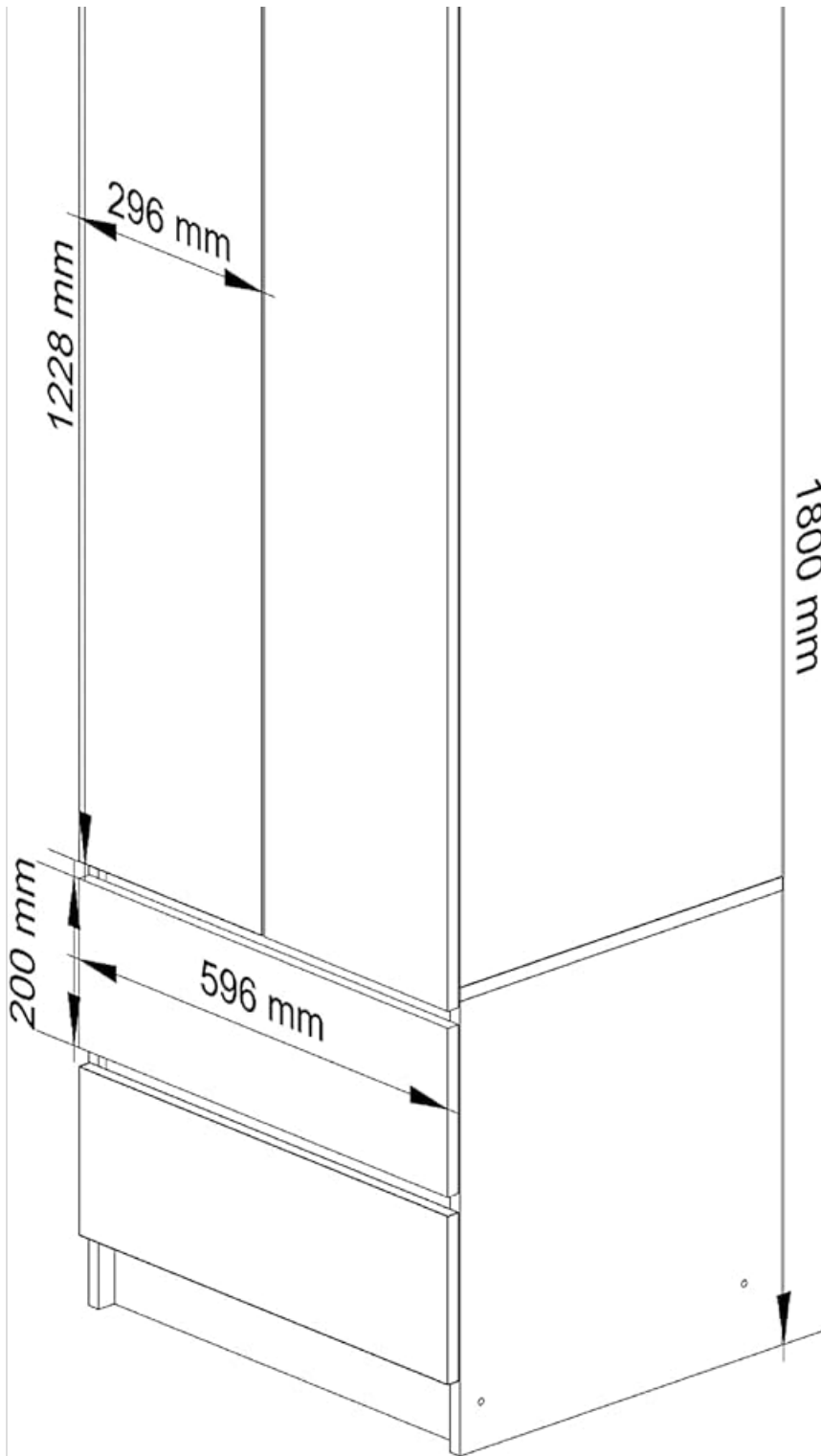
Figure 1: Technical drawing illustrating the dimensions of the AKORD S60 wardrobe, including the main unit and the 60 cm extension. Key measurements such as height, width, and depth are indicated in millimeters, providing a detailed overview for assembly and placement.
