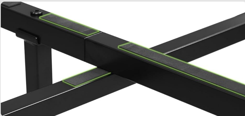
Image 4.1: Visual representation of the bed frame's strong structural design, the snap-in slat system for easy assembly, and the EVA silent rod for noise reduction.
