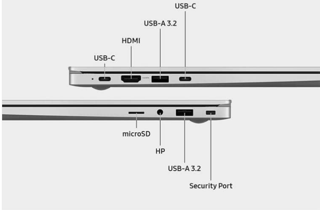
Figure 3: Side view of the laptop highlighting the various input/output ports for connecting peripherals and external displays.
