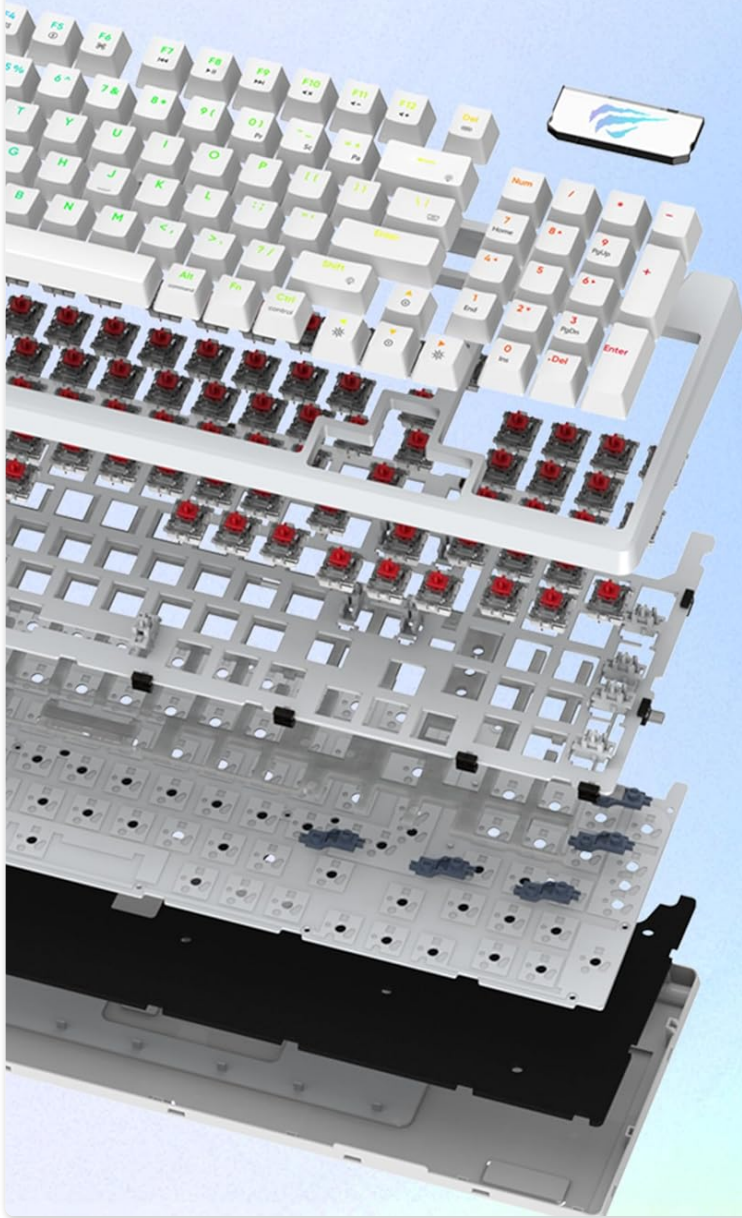
Image: An exploded view of the Havit Gamenote KB885L keyboard, illustrating its internal gasket structure for enhanced stability and typing feel.
