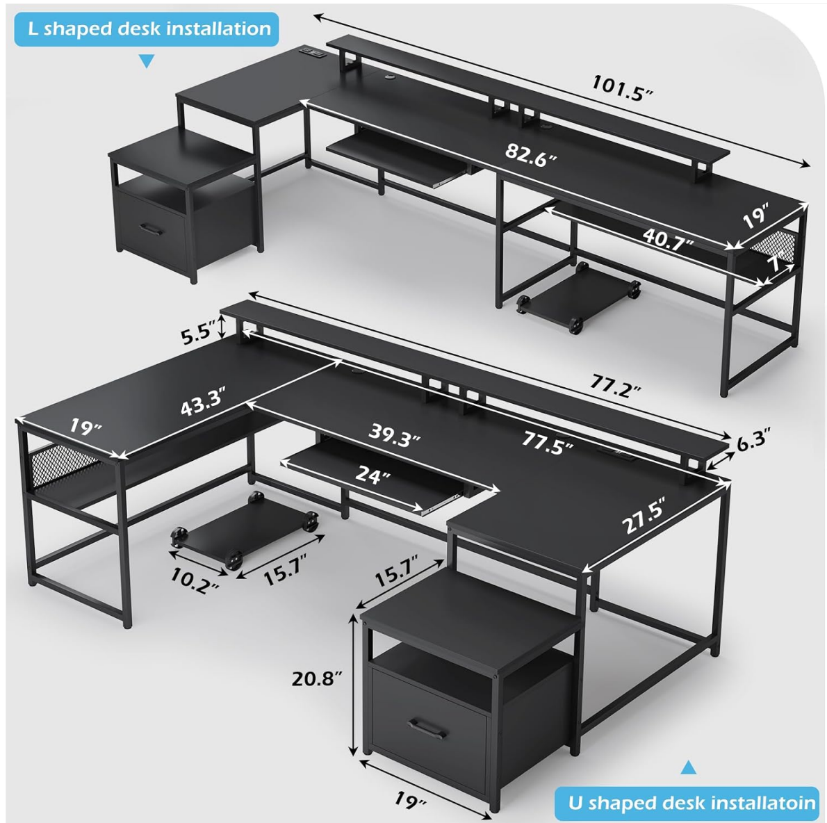
Image: Diagram showing the dimensions of the L-shaped and U-shaped desk configurations, illustrating the various components and their sizes.
