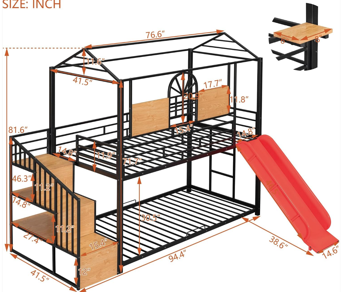
Image: A technical diagram illustrating the precise dimensions of the bunk bed, including length, width, height, and specific measurements for the slide, stairs, and bed levels.
