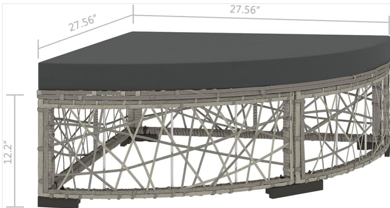
Figure 6: Detailed dimensions for the fan shape footrest.
