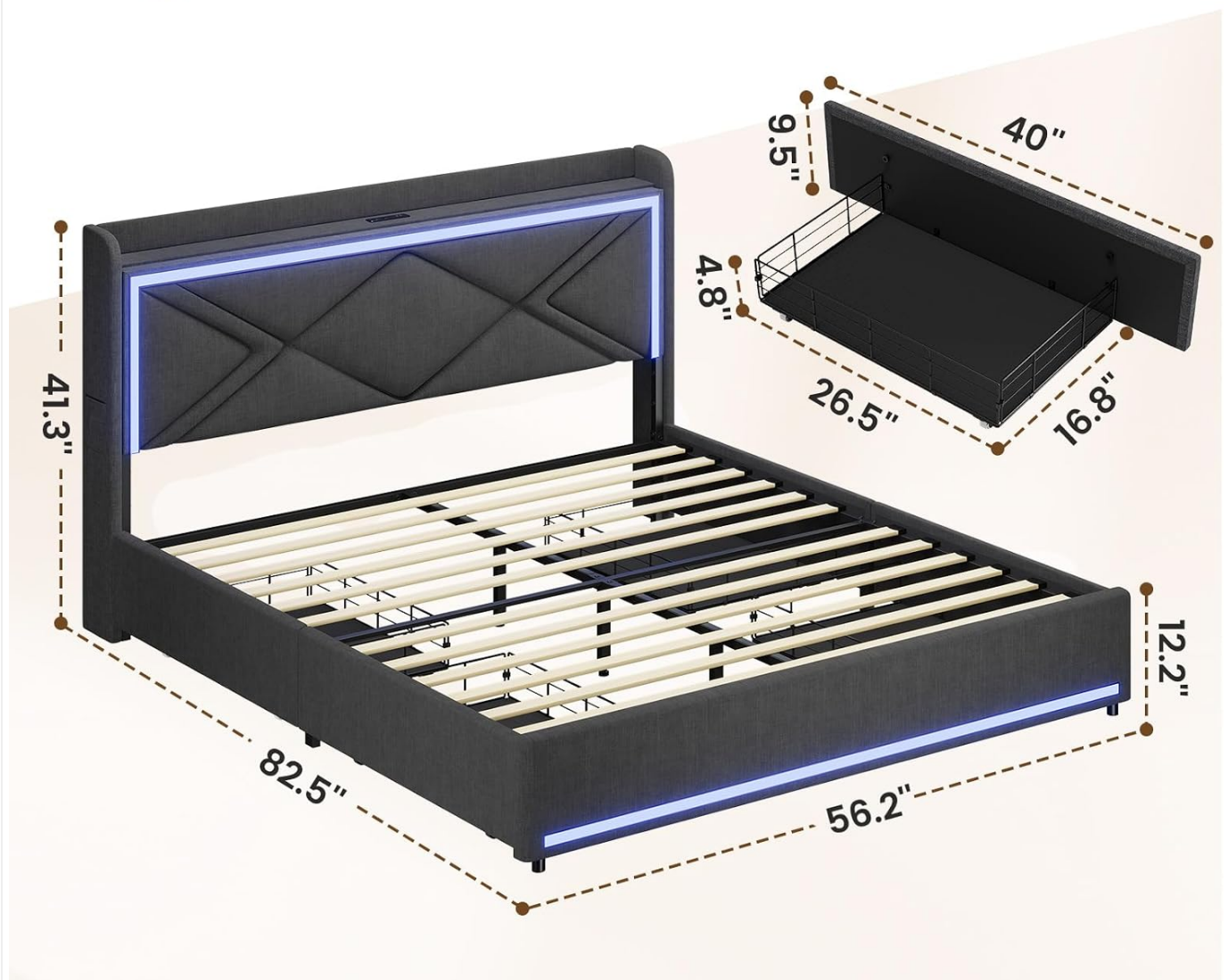
Image 3.1: Overview of bed frame dimensions and maximum weight capacity.
