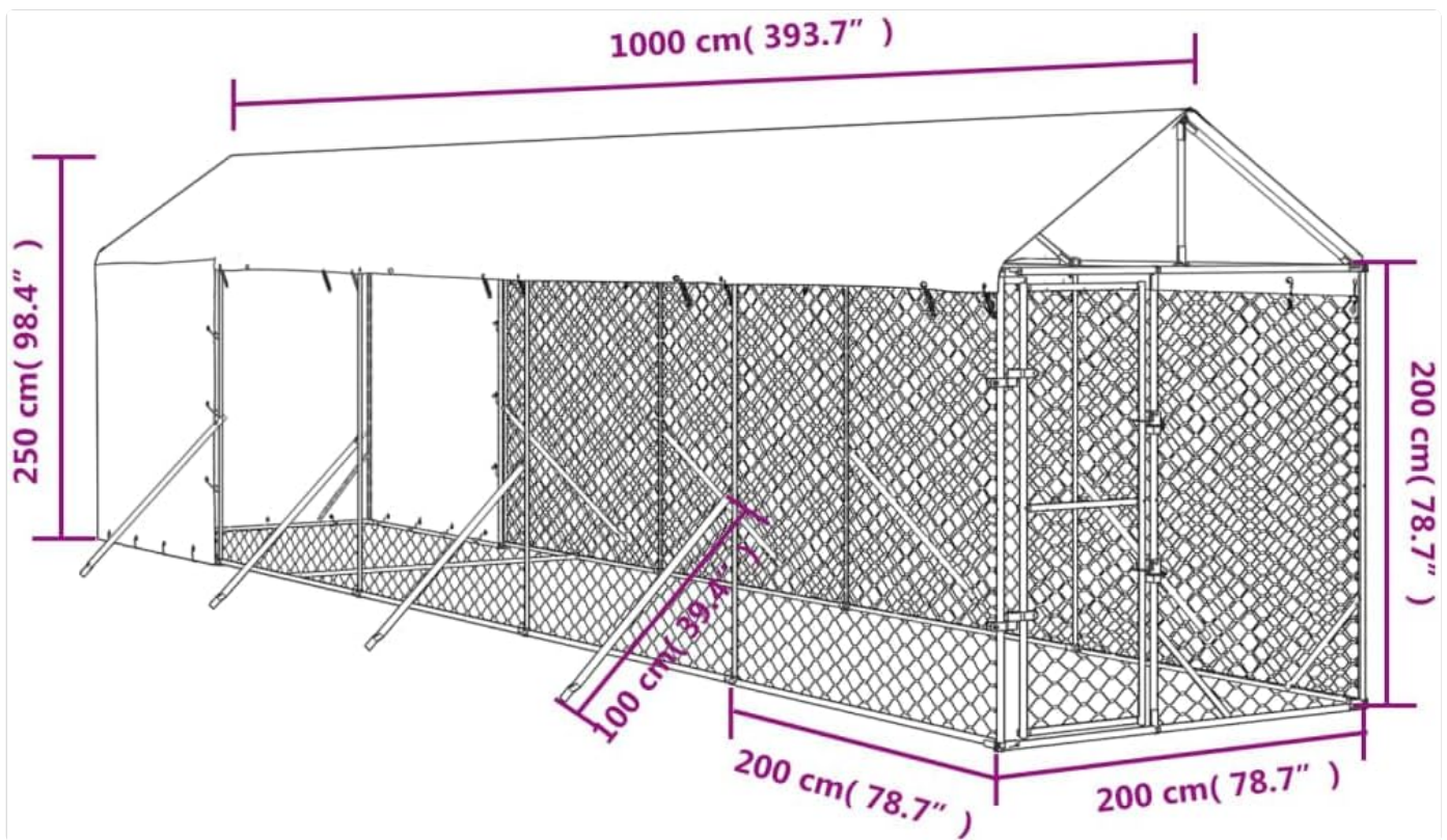
Image 8.1: Detailed dimensions of the kennel structure. This diagram illustrates the overall length, width, and height, including specific measurements for various sections.
