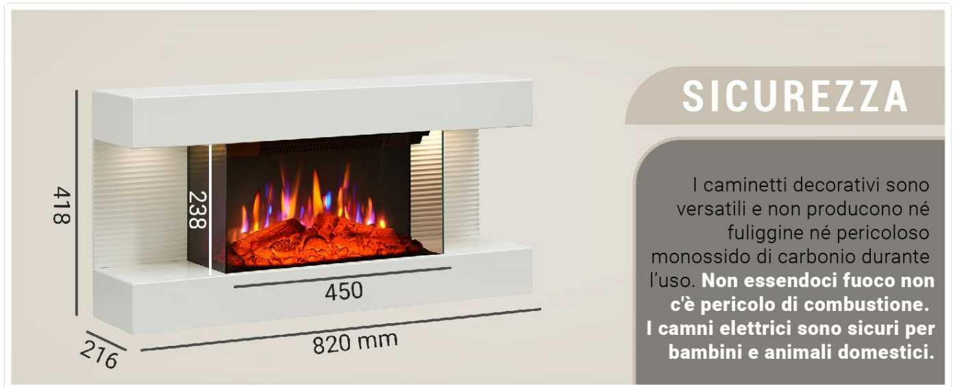
Diagram showing the dimensions of the BALDERIA Ida electric fireplace with safety information.
