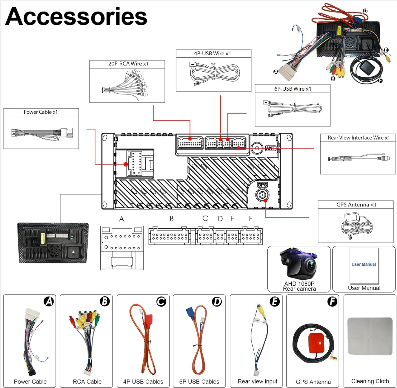
Image: Overview of included accessories and wiring connections.
