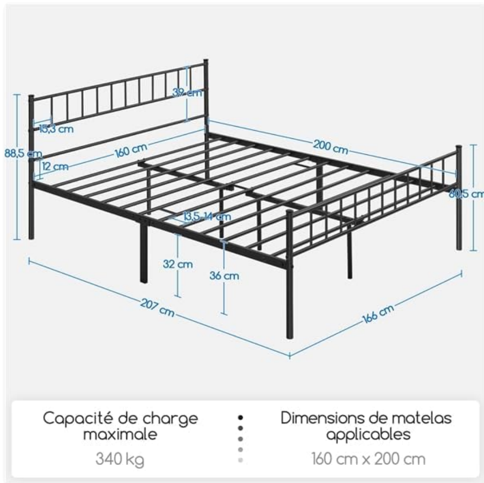
Image 8.1: Dimensional overview of the bed frame.
