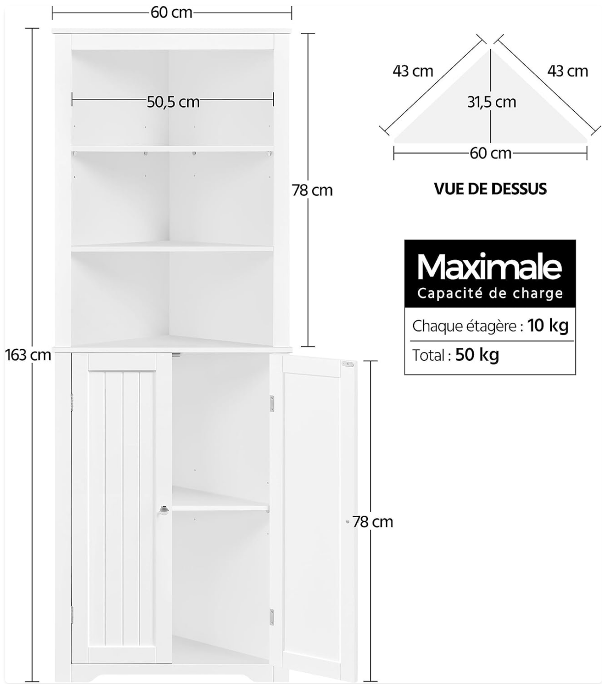
Image 8.1: Detailed dimensions and maximum load capacity for the cabinet.
