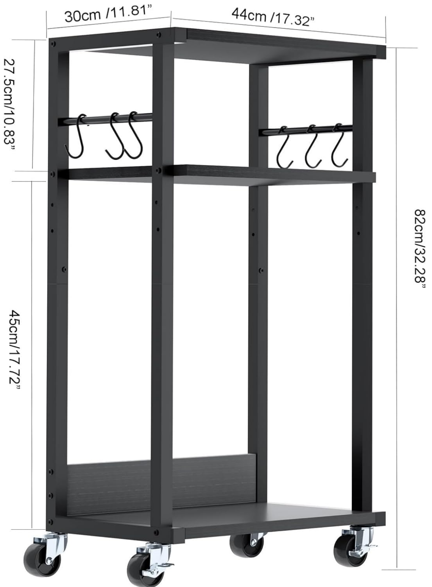
Image: A technical drawing illustrating the precise dimensions of the printer stand in both centimeters and inches.
