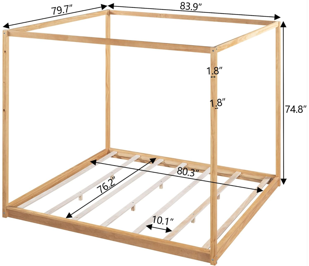
Image: A detailed diagram illustrating the key dimensions of the bed frame, including length, width, and height, in inches.
