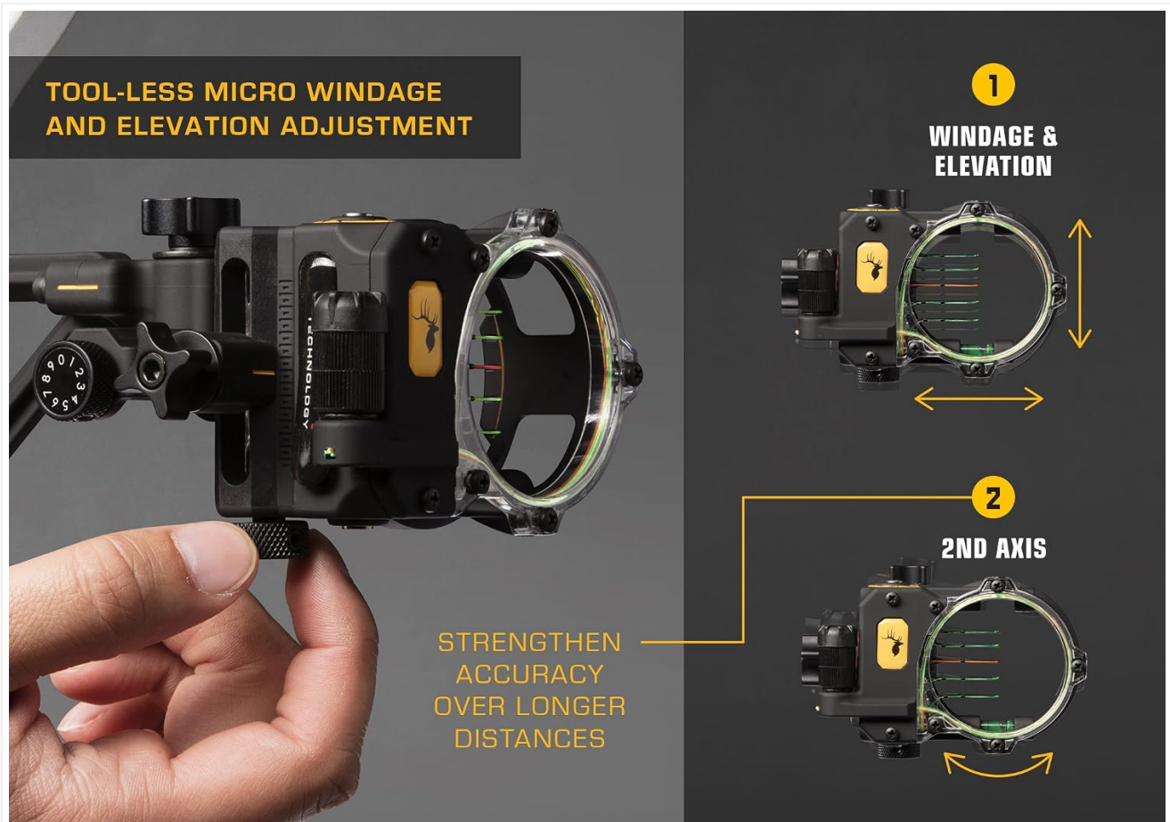
Image: Detailed view of the sight highlighting the tool-less micro windage and elevation adjustments and the 2nd axis leveling mechanism.
