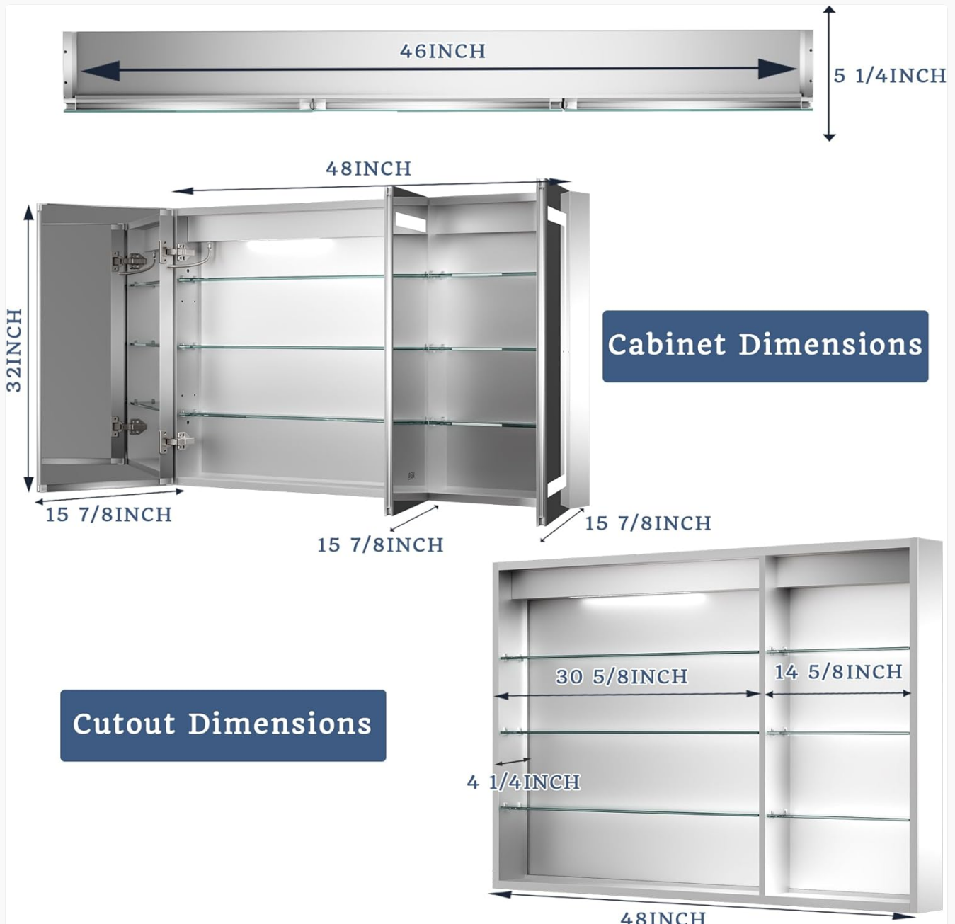
Figure 2: Cabinet and Cutout Dimensions (48x32 Inch model)
