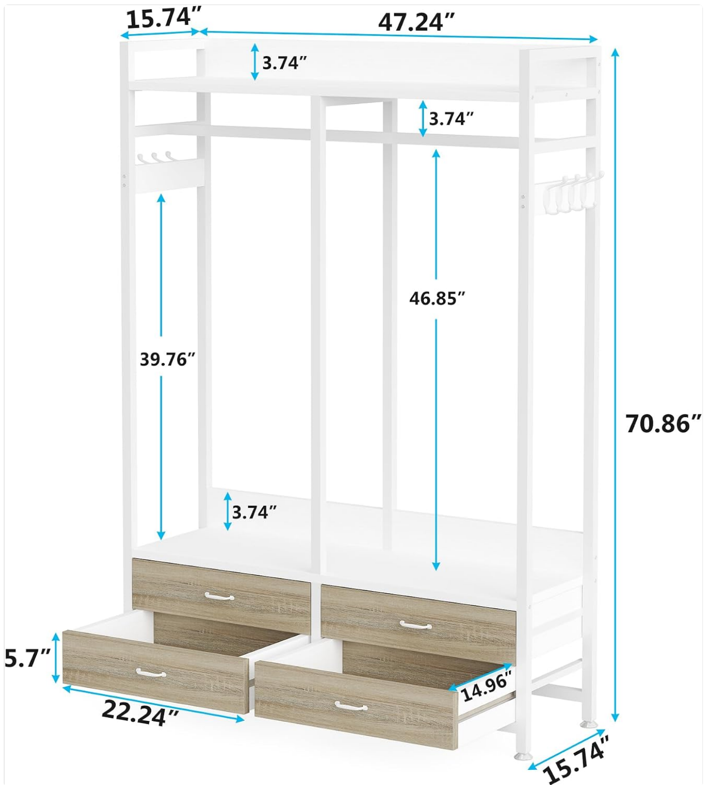
Image: Dimensional diagram of the closet organizer, providing key measurements for planning placement.
