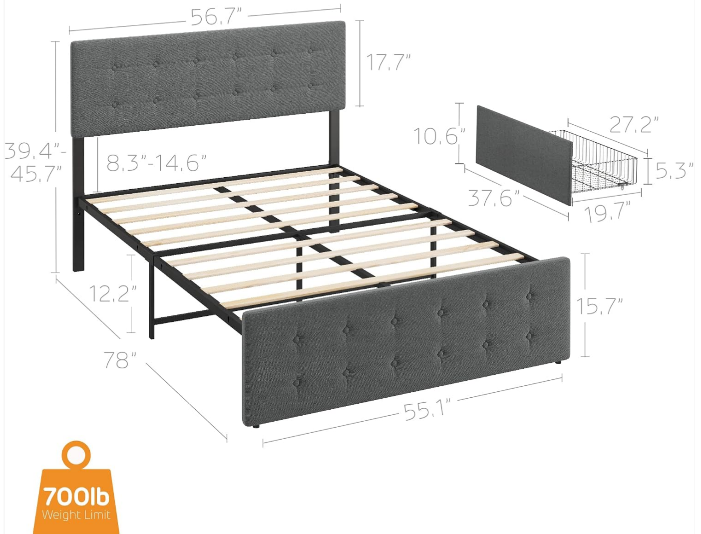
Image: Full product dimensions diagram.
