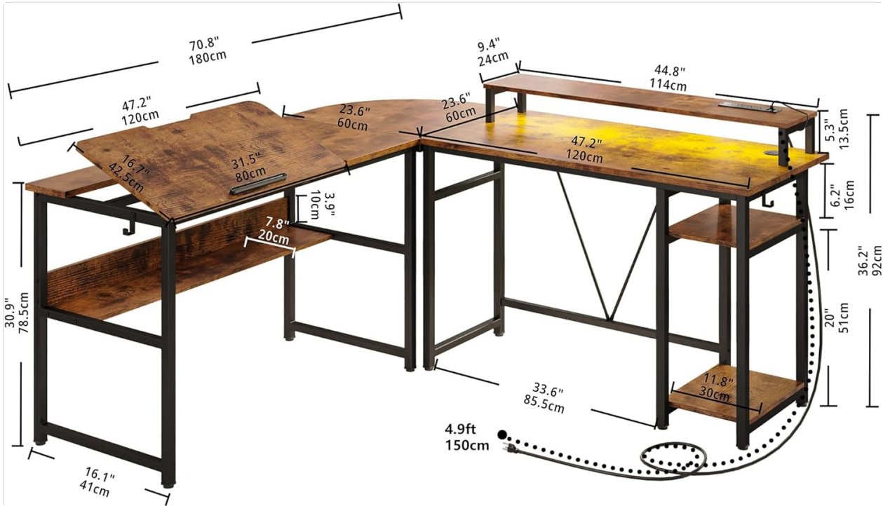
Figure 1: Desk Dimensions. This diagram illustrates the overall measurements of the L-shaped desk, including the length of each segment and the depth, crucial for planning your space.
