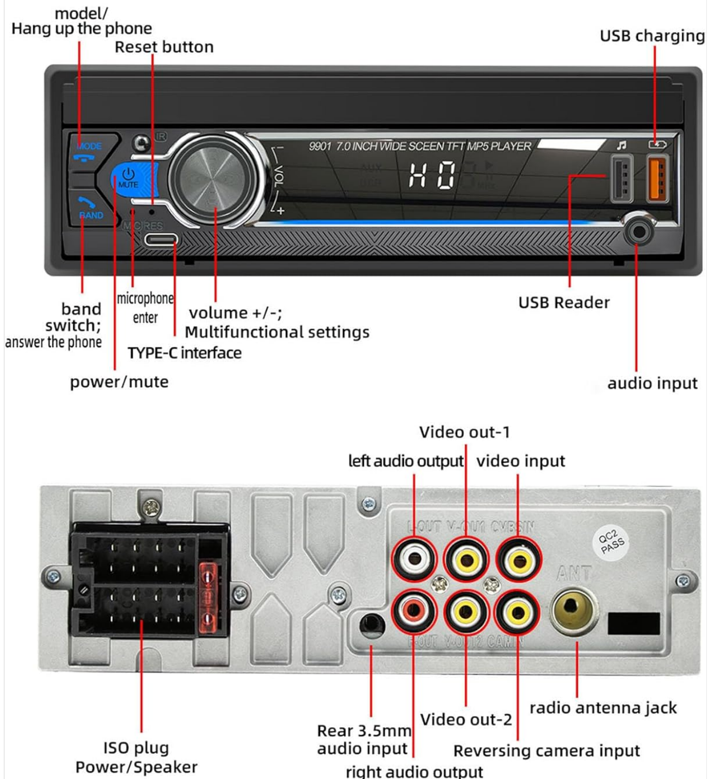
Figure 3.2: Detailed diagram labeling the various buttons, ports, and connectors on both the front panel and the rear panel of the car MP5 player.
