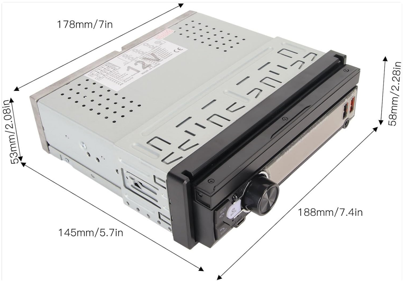
Figure 3.1: Diagram illustrating the dimensions of the car MP5 player unit, including width, height, and depth.
