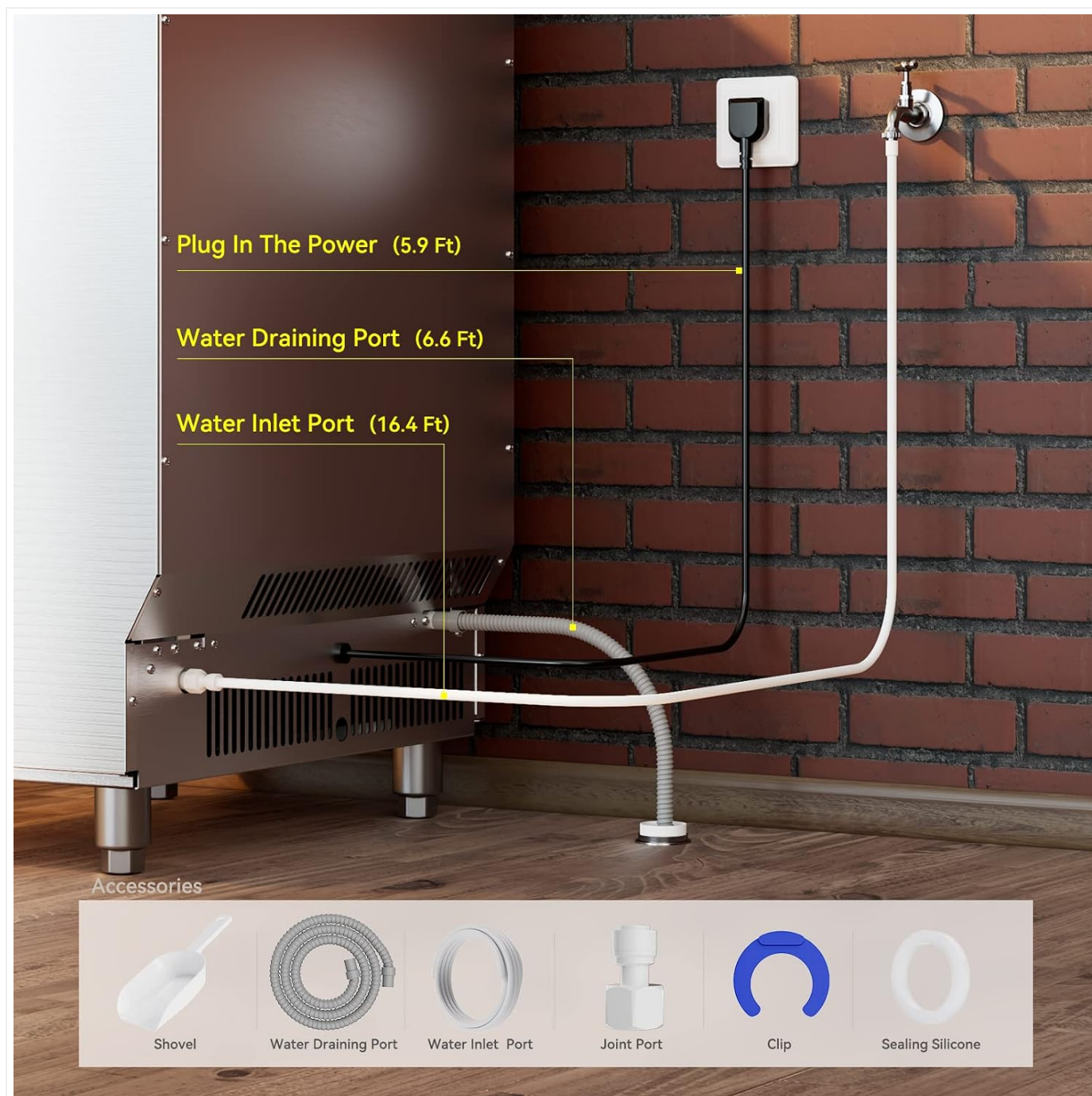
Image: Rear view of the ice maker showing the power plug, water draining port (6.6 ft), and water inlet port (16.4 ft) connections. Essential accessories like a shovel, water draining port hose, water inlet port hose, joint port, clip, and sealing silicone are also shown.
