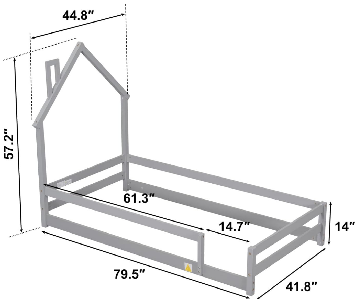
Image 8.1: Dimensional diagram of the LLS Twin Size Floor Bed, indicating key measurements.
