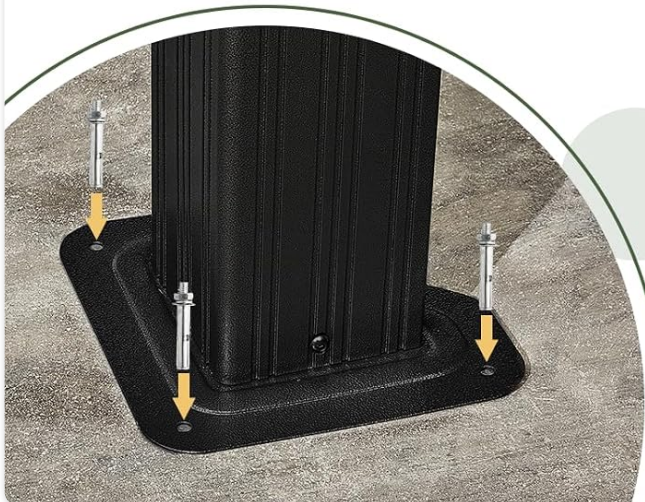
Figure 3.1: Illustration of the sturdy aluminum frame, highlighting the Interpon AkzoNobel powder coating, solid triangular structure, and anchoring frame for enhanced stability.
