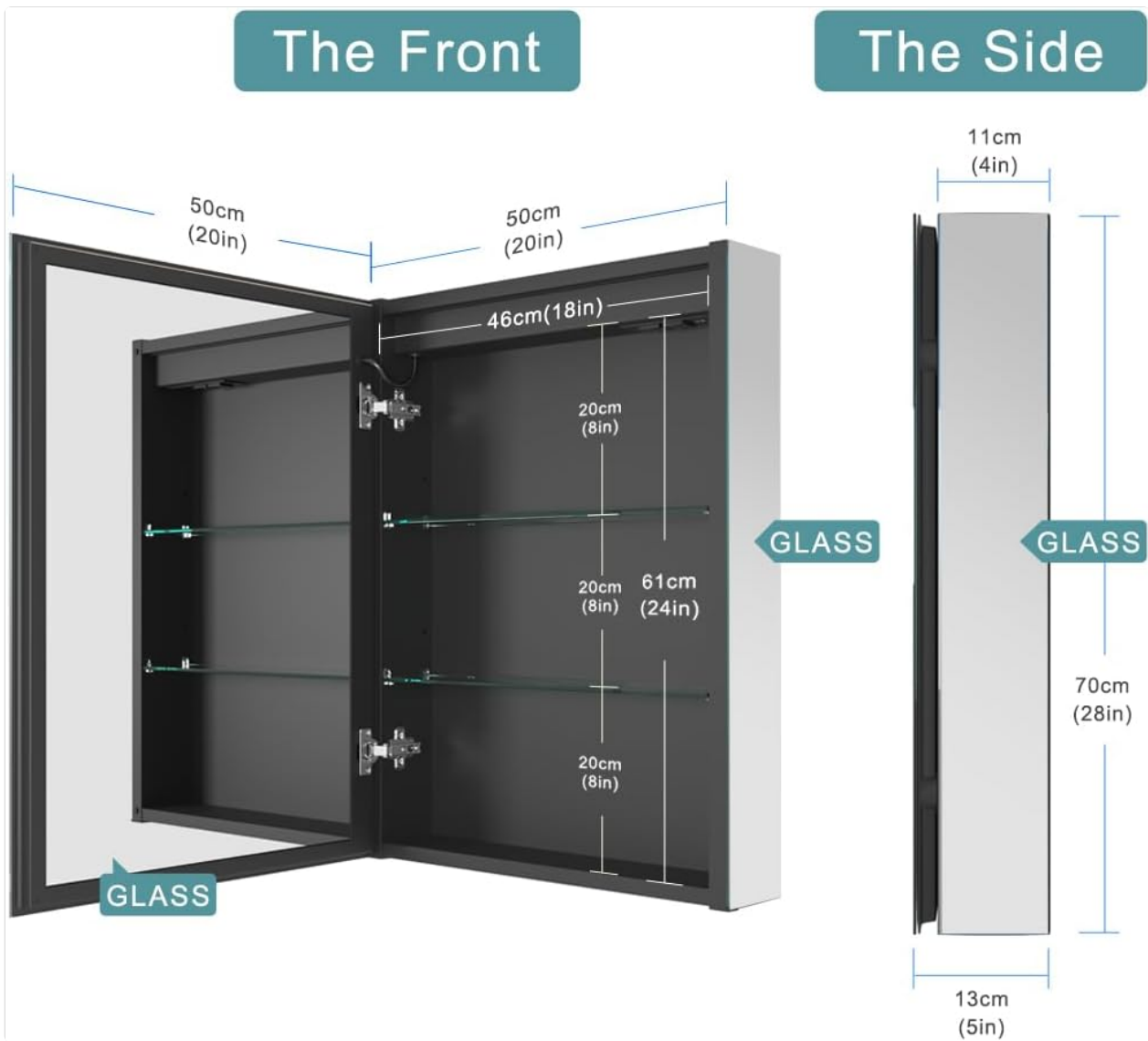
Figure 4.1: Detailed dimensions of the GANPE Medicine Cabinet.
