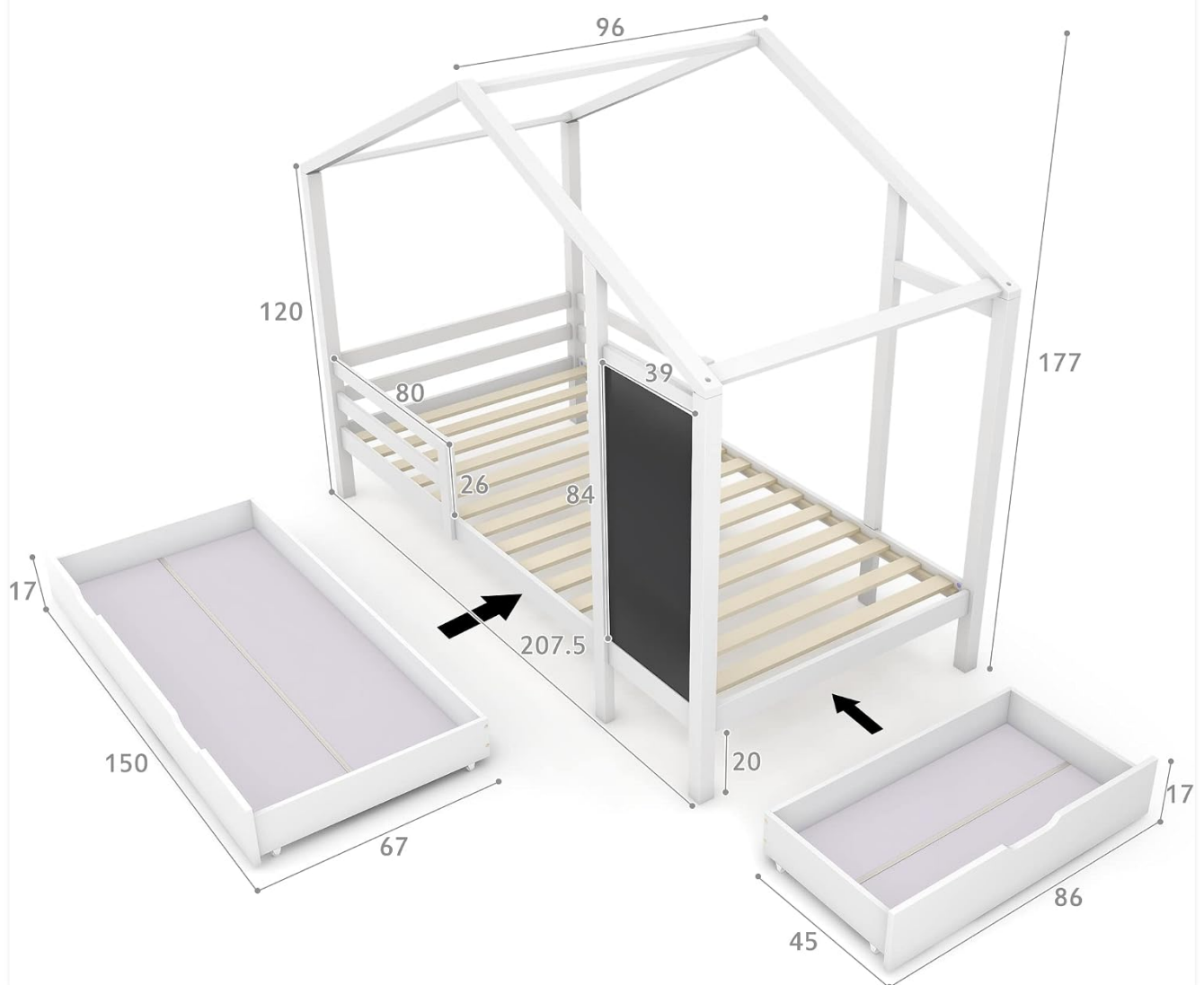
Figure 3: Detailed dimensions and component layout for assembly
