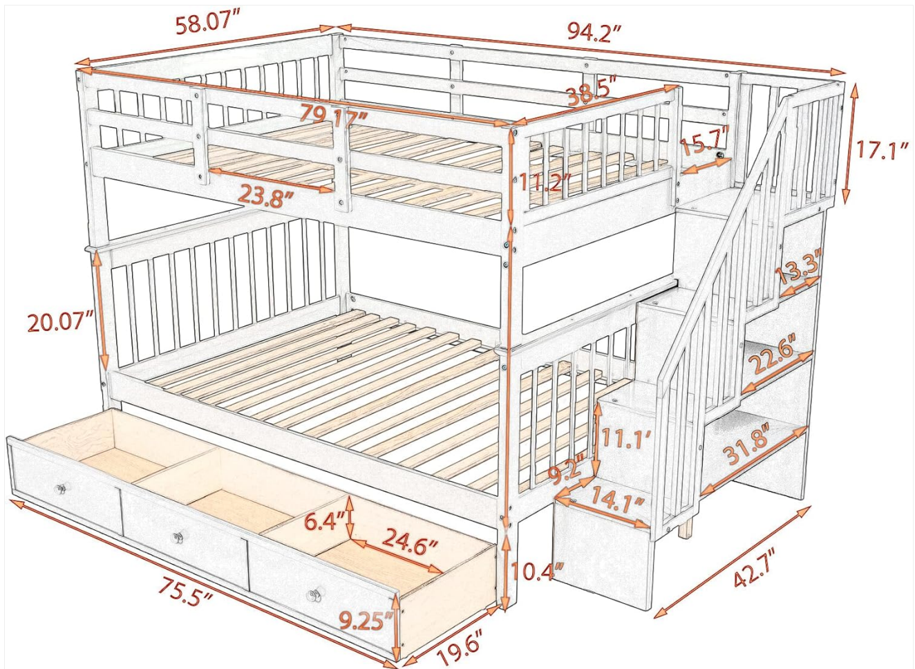
Image 4.1: Detailed dimensions of the bunk bed, including overall length, width, height, and individual component measurements.
