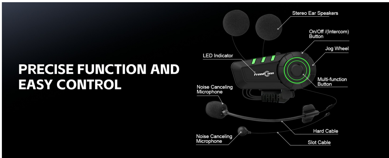
Image: A detailed diagram showing the precise functions and easy controls of the FreedConn KY headset, including the LED indicator, On/Off/Intercom button, Jog Wheel, Multi-function Button, Noise Canceling Microphone, Hard Cable, and Slot Cable.
