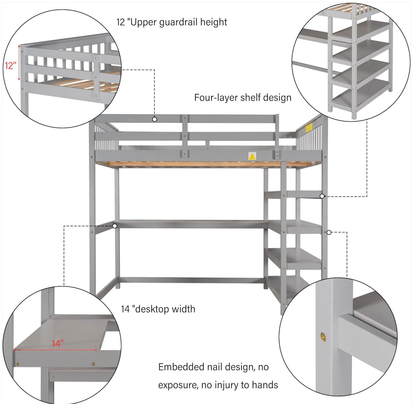
Image: Detailed view highlighting the 12-inch guardrail, four-layer shelf design, 14-inch desktop width, and embedded nail design for safety.
