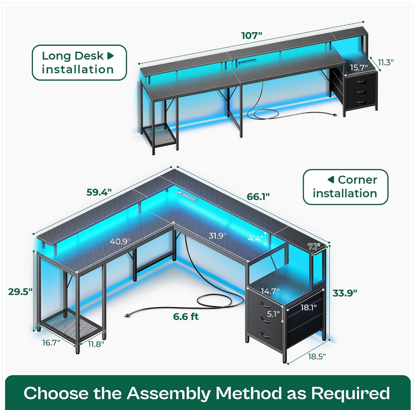
Figure 2: Detailed dimensions for both the L-shaped corner installation and the long desk installation, illustrating the flexibility in setup.
