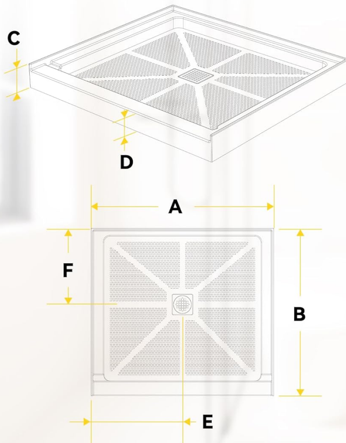
Figure 7: Detailed dimensions of the Sunrosa 36x36 shower base.
