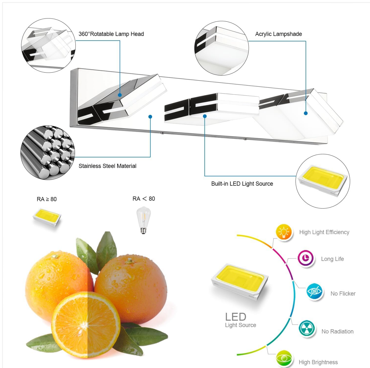
Image 2: Component diagram of the SineRise Vanity Light, highlighting the rotatable lamp heads, acrylic lampshade, stainless steel material, and built-in LED light source.
