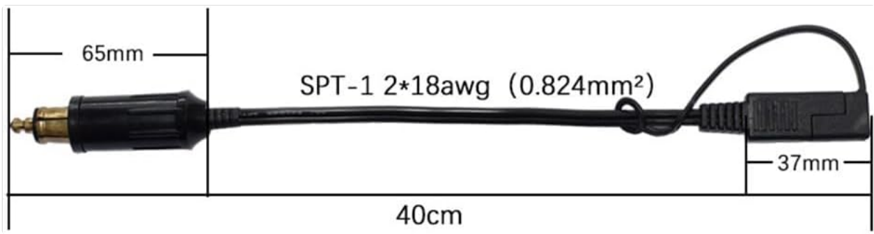
Figure 8.1: Approximate dimensions of the ZYNCUE Motorcycle Connection Cable.
