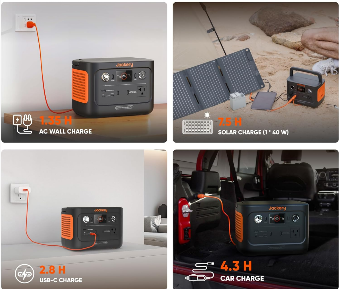
Figure 5.1: Visual representation of the four primary charging methods for the Explorer 300 Plus.
