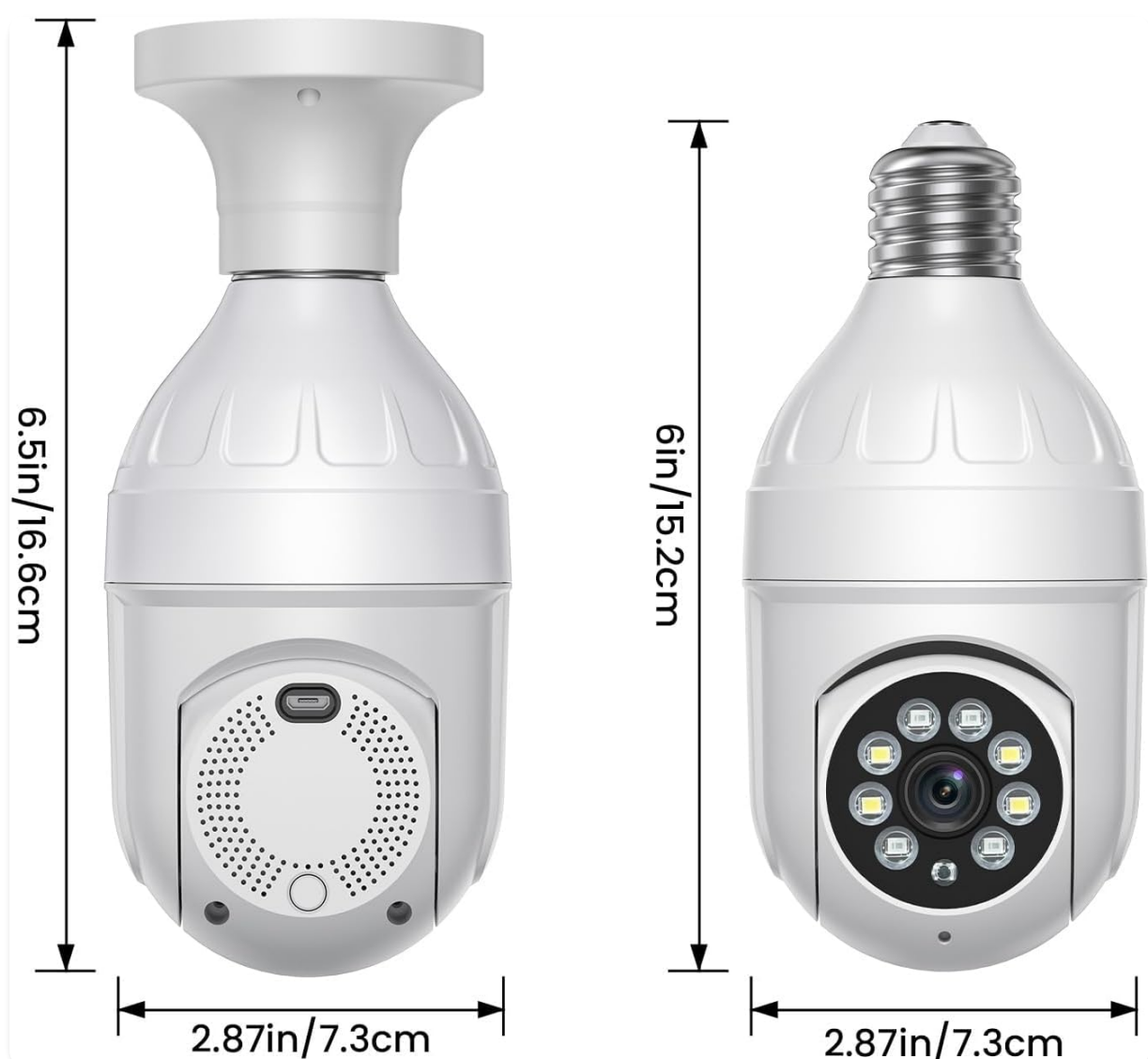
Image: Detailed dimensions of the SHARKPOP Light Bulb Security Camera.
