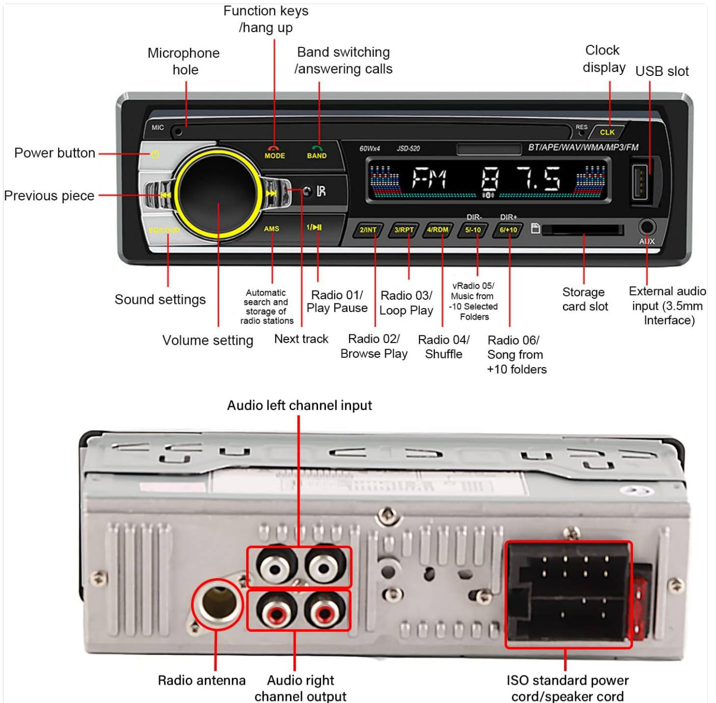
Figure 2: Front Panel Layout. This diagram shows the location of the power button, microphone hole, function keys, band switching, volume setting, sound settings, automatic search and storage of radio stations, play/pause, loop play, browse play, shuffle, folder navigation, clock display, USB slot, storage card slot, and external audio input (AUX).
