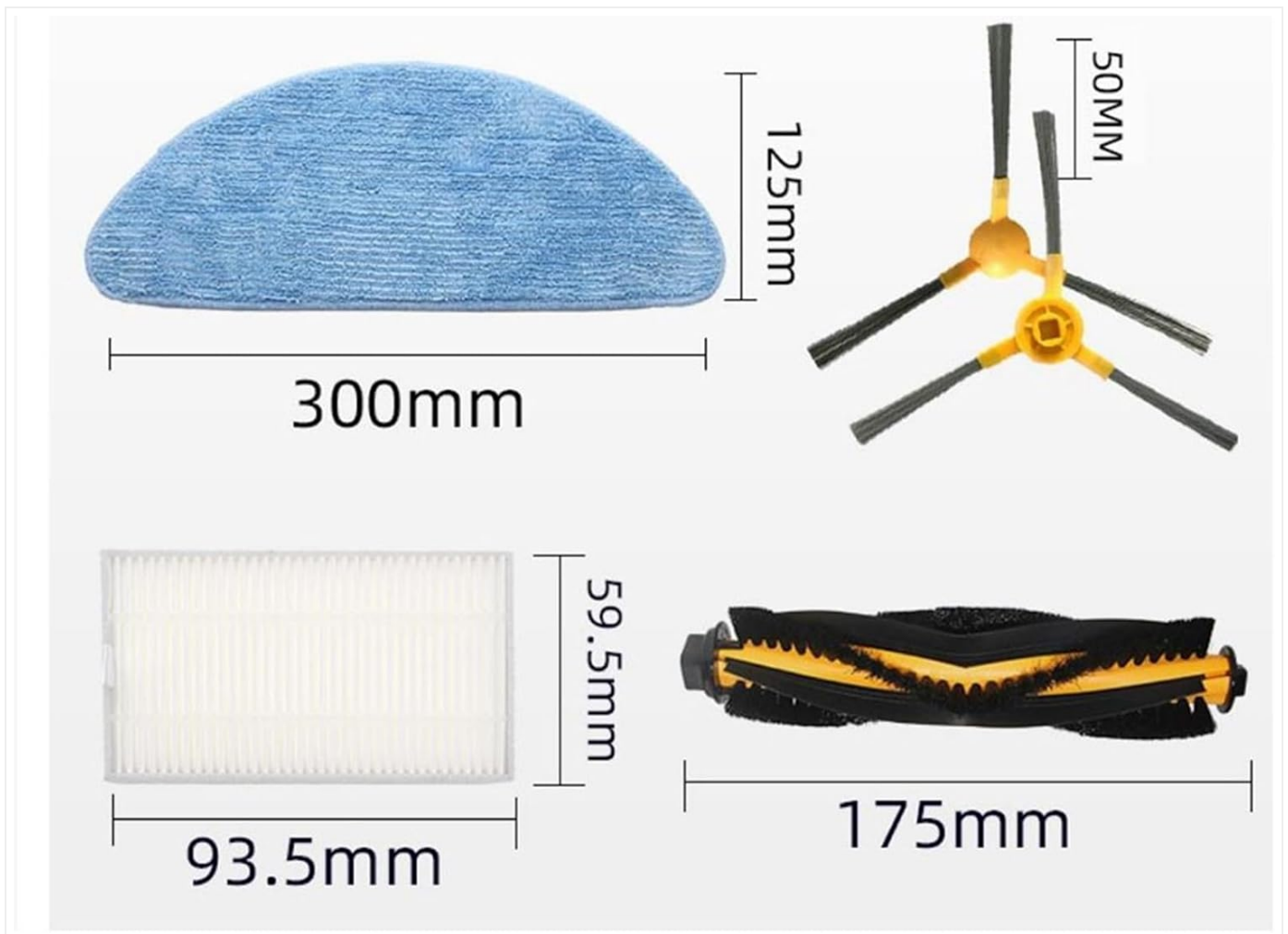
Image: Dimensional diagram illustrating the approximate sizes of the mop pad, side brush, HEPA filter, and main brush for compatibility reference.
