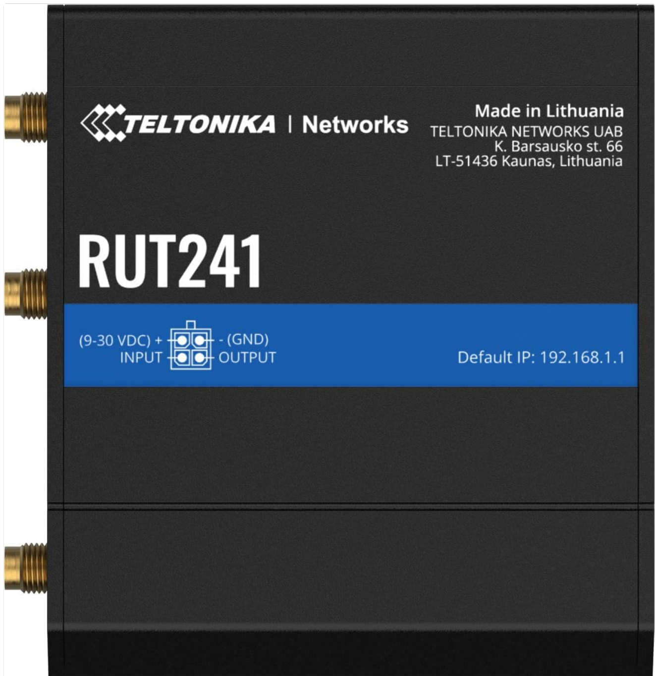
Figure 4.1: Front view of the RUT241 router, displaying the model number, Teltonika branding, power input specifications (9-30 VDC), and the default IP address (192.168.1.1).
