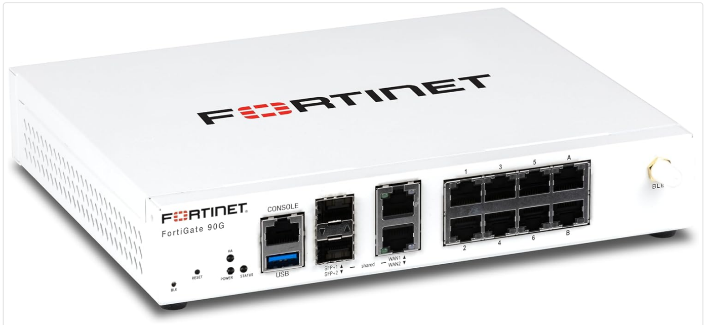
Figure 2.3: Close-up of the FortiGate 91G front panel, detailing the console, USB, SFP+, WAN, and Ethernet ports.
