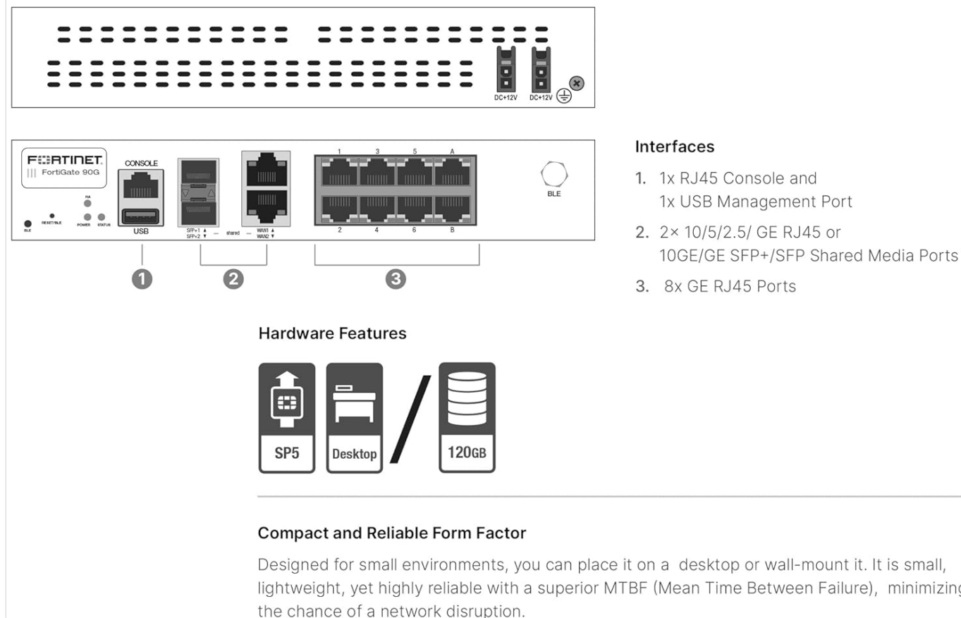
Figure 2.4: Diagram illustrating the interfaces of the FortiGate 90G. This includes the RJ45 Console and USB Management Port, 2x 10GE/GE SFP+ Shared Media Ports, and 8x GE RJ45 Ports.
