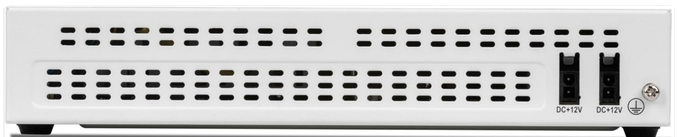
Figure 2.3: Rear view of the FortiGate 90G, showing the dual DC+12V power inputs and grounding screw.
