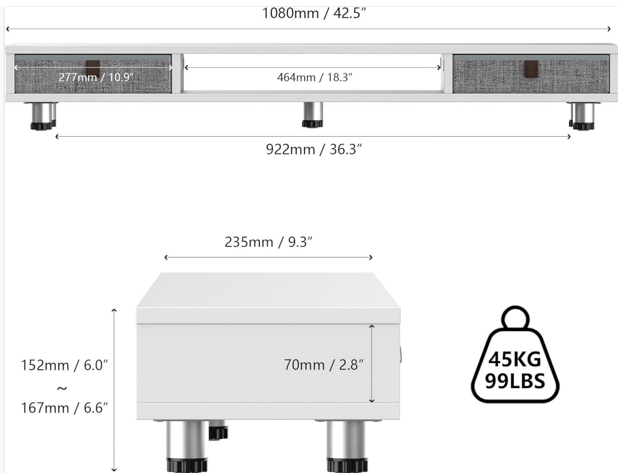
Image 6.1: Detailed dimensions and weight capacity of the monitor stand.
