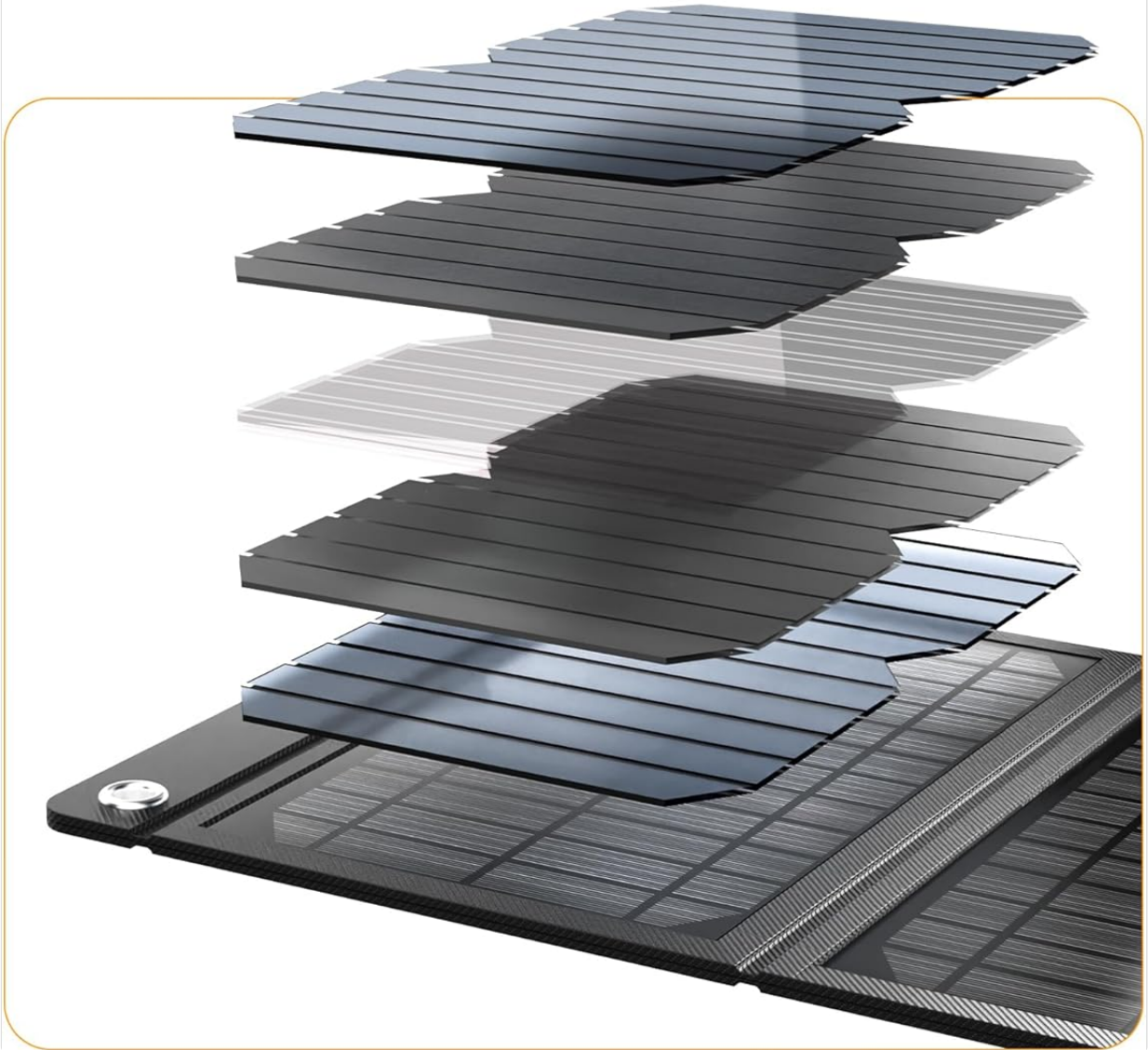
Image: An exploded view diagram showing the layers of the solar panel, emphasizing its 23% efficiency and protective features like dust-proof, abrasion resistance, and waterproofing.
