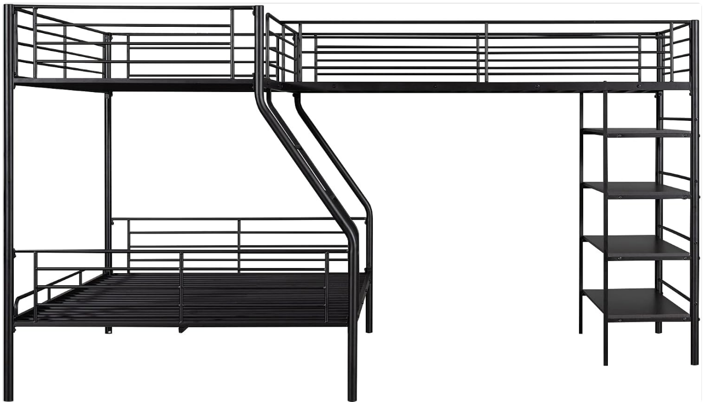
Image: A detailed view of the L-shaped configuration, highlighting the connection points and the integrated shelving unit, crucial for assembly reference.
