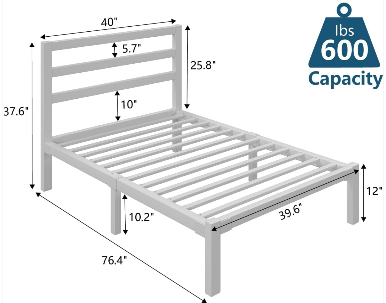
Figure 8.1: Detailed dimensions and weight capacity of the Twin Size bed frame.
