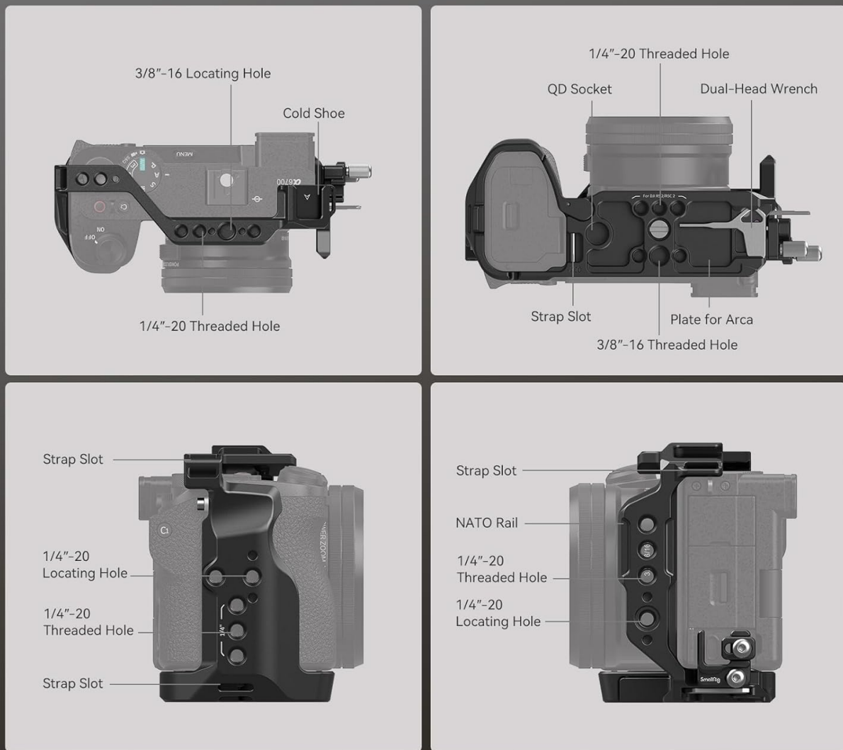
Figure 4.2: Overview of mounting points for accessories.
