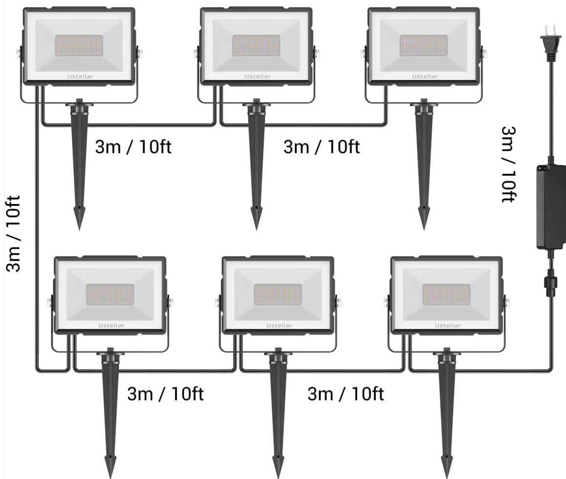
Image: A clear diagram illustrating the series connection of six floodlights to a single power adapter, highlighting the 10ft (3m) cable length between each light for a total of 60ft (18m).
