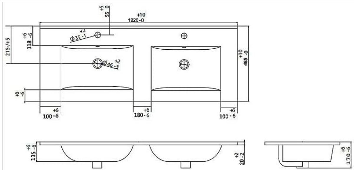
Image 4.1: Technical drawing illustrating the dimensions and layout of the MOTIAC integrated sink.
