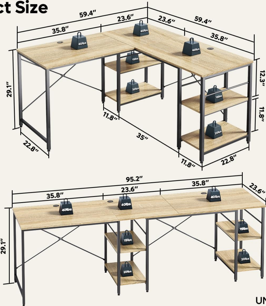
Figure 2: Desk dimensions and reversible configurations.
