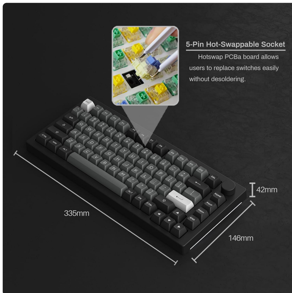
Image: Detailed view of the 5-pin hot-swappable sockets for easy switch replacement.
